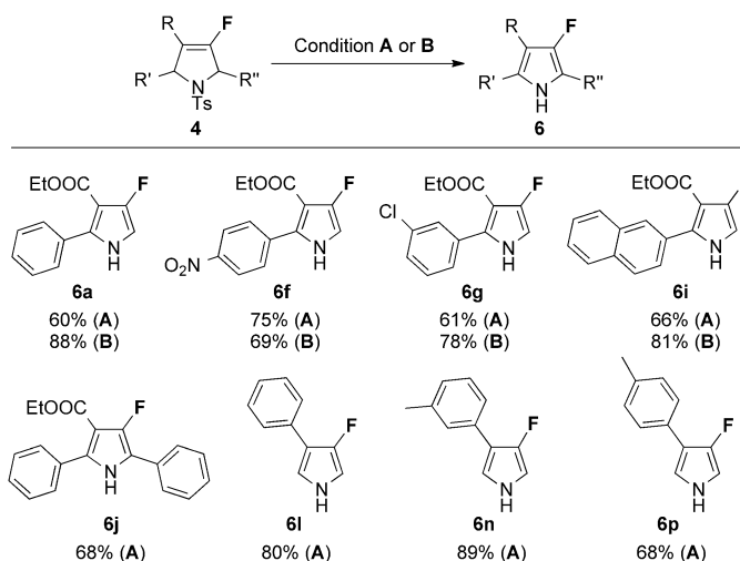
Scheme 3. The aromatization of 4-fluoro-2,5-dihydropyrroles. Condition A: \text{KO}^t\text{Bu} (3 equiv), DMSO, RT or 50°C for 2 h; Condition B: 1) DDQ (3 equiv), benzene, 110°C, 5 h; 2) \text{EtONa} (5 equiv), EtOH, 30°C, 1 h. The yields of isolated product are given.
