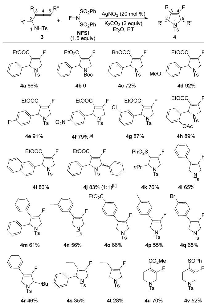
Scheme 2. Silver-catalyzed aminofluorination of allenes. Reaction conditions were the same as for Table 1, entry 7. The yields of isolated product are given. [a] NFSI (3 equiv) and \text{K}_2\text{CO}_3 (4 equiv). [b] Starting material 3j is a mixture of two isomers (d.r. 1:1). Bn = benzyl, Boc = tert -butoxycarbonyl.
